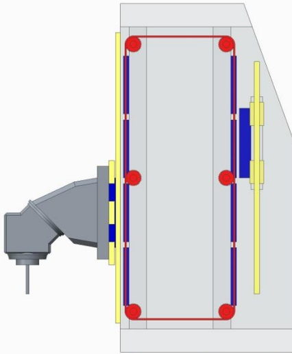
Design concept with belt-coupling
