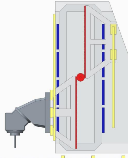
Design concept with rack-and-pinion
